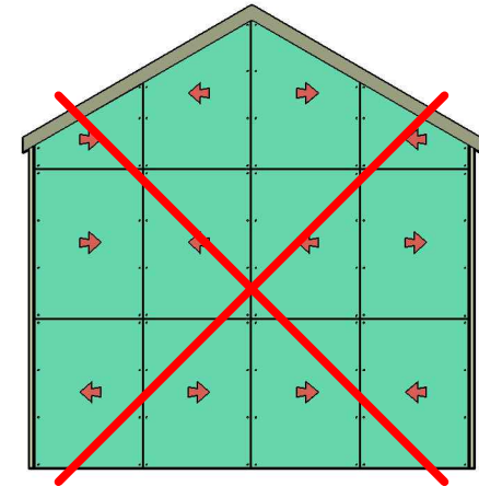
IMPROPER PANEL LAYOUT TECHNIQUE
