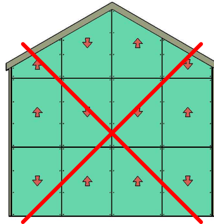
IMPROPER PANEL LAYOUT TECHNIQUE
