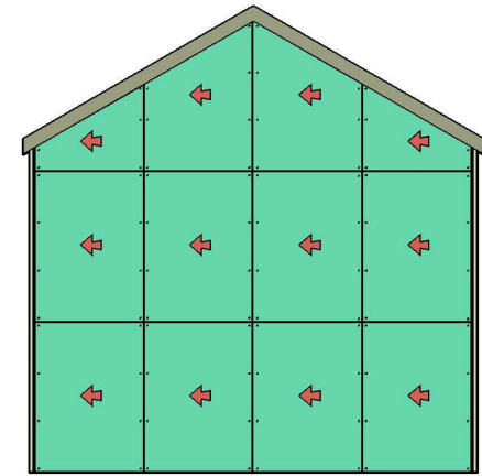
PROPER PANEL LAYOUT TECHNIQUE
